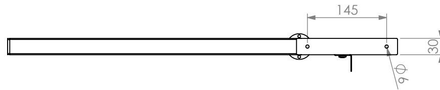
PLAN VIEW
