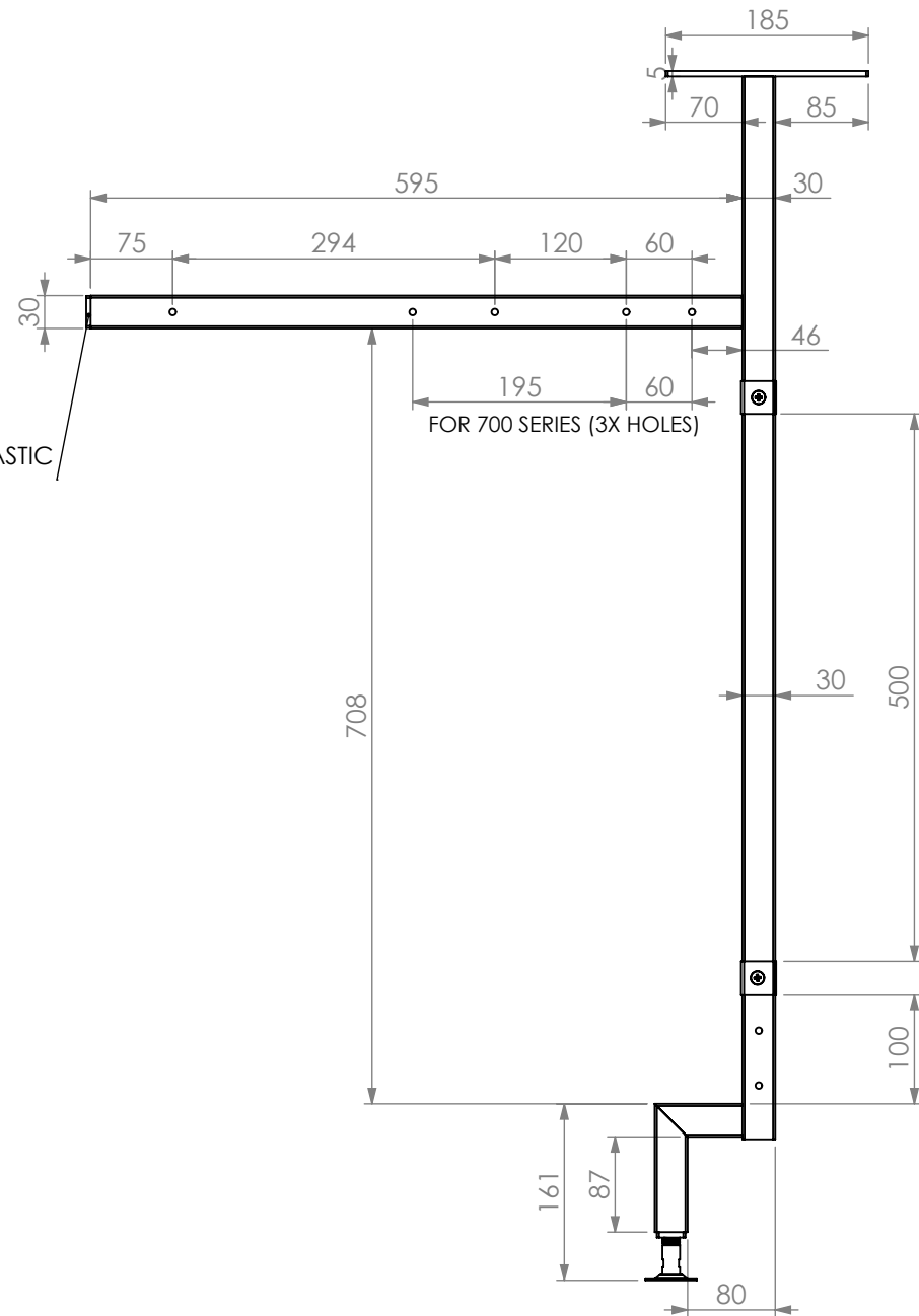
SIDE ELEVATION
